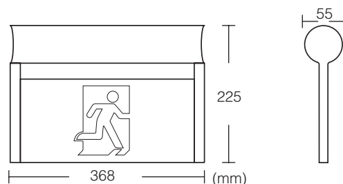
AQUA LOCK-W (IP65) with LED Blade
