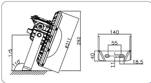
Stanchion Mount
