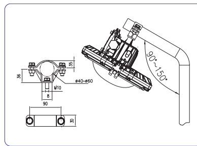
Pipe Clamp
