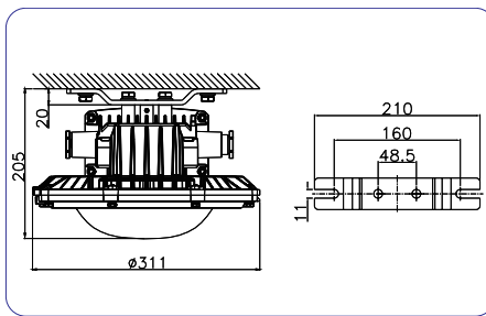
Ceiling Mount
